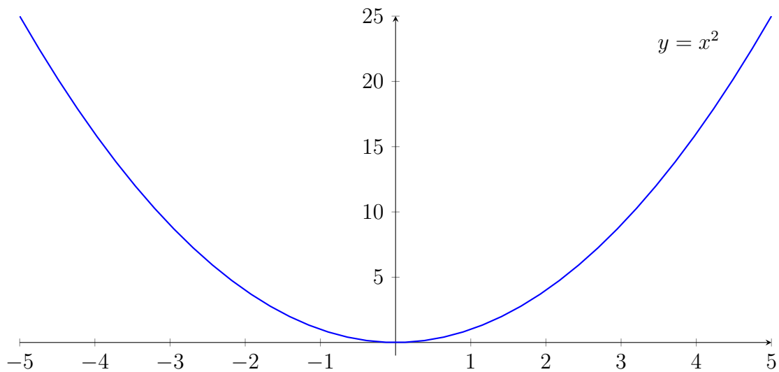
Figure 1: A graph of a quadratic.
